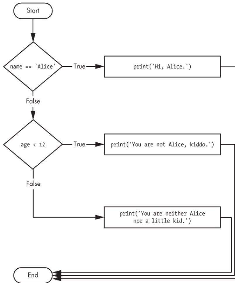
Figure 2-7: Flowchart for the previous littleKid.py program
