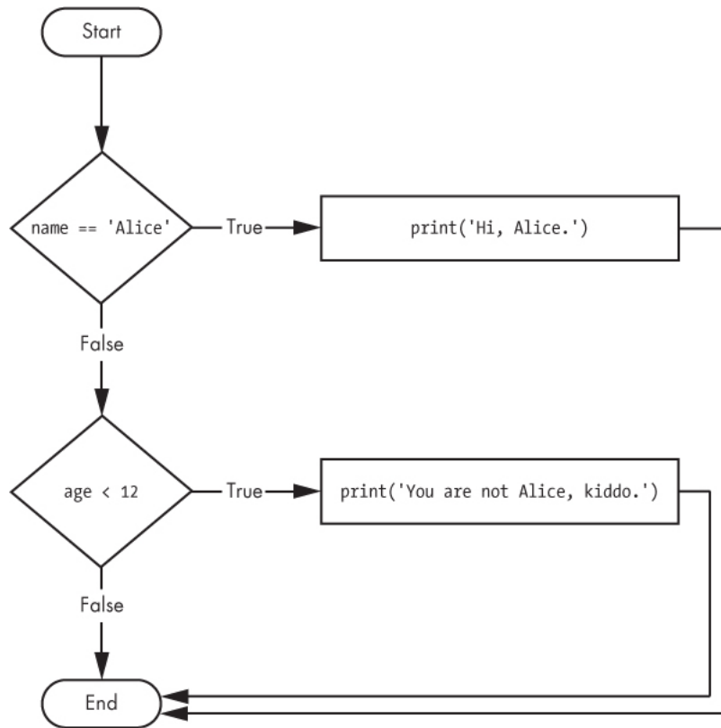
Figure 2-4: The flowchart for an elif statement
