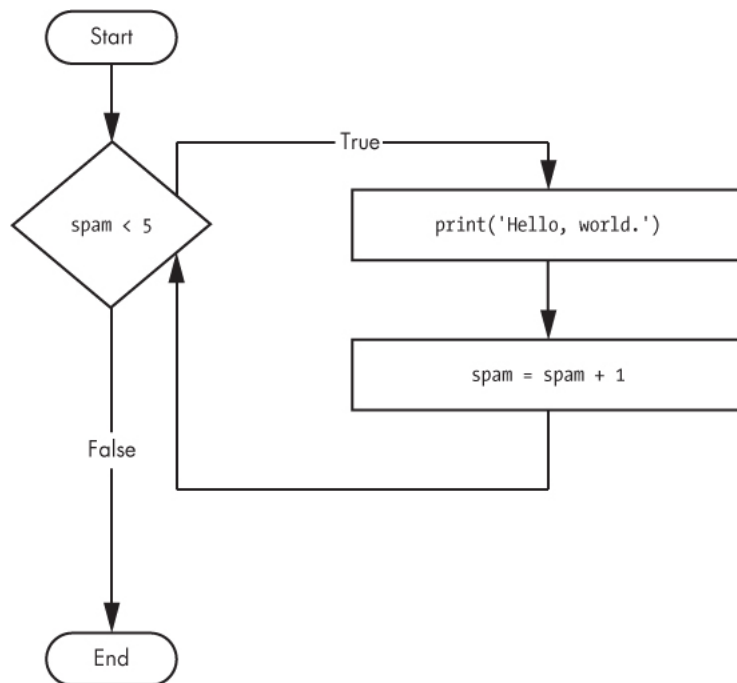
Figure 2-9: The flowchart for the while statement code
