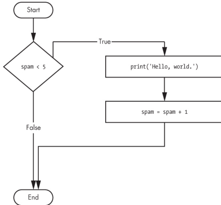
Figure 2-8: The flowchart for the if statement code
